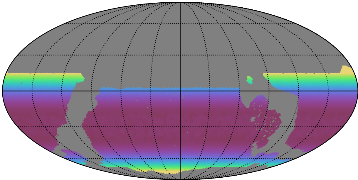
weather_cloudso2v3.4_10yrs WFD all bands: Min airmass
