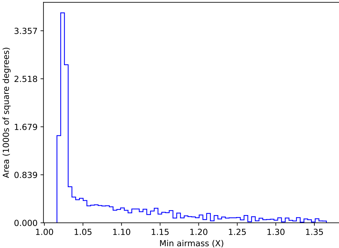
weather_cloudso2v3.4_10yrs WFD all bands: Min airmass
