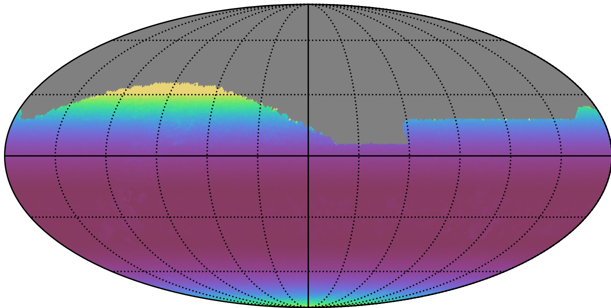
weather_cloudso2v3.4_10yrs All sky z band: Min airmass
