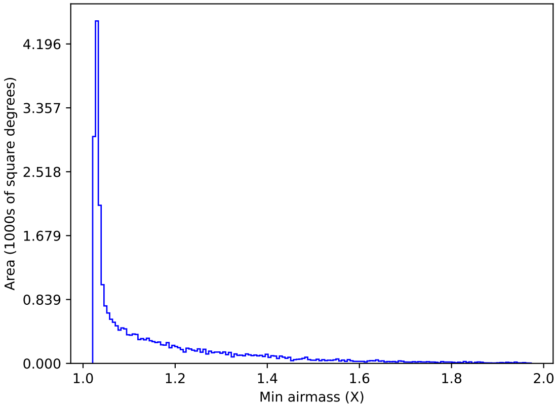
weather_cloudso2v3.4_10yrs All sky z band: Min airmass
