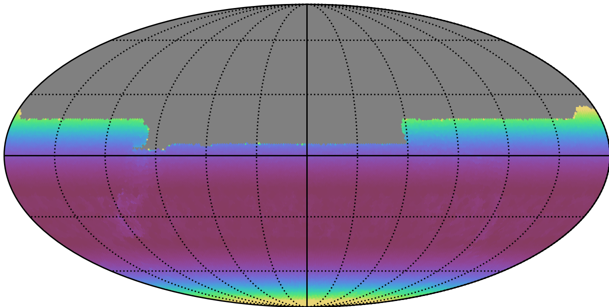
weather_cloudso2v3.4_10yrs All sky y band: Min airmass
