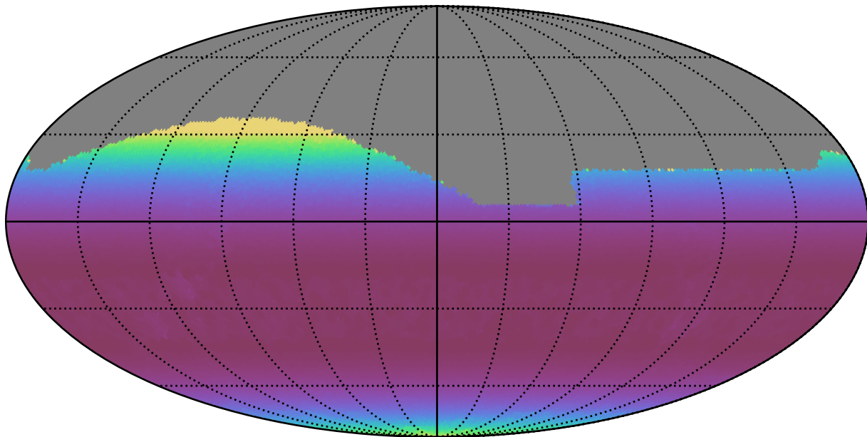
weather_cloudso2v3.4_10yrs All sky g band: Min airmass
