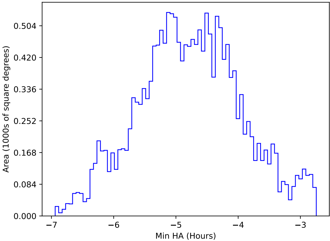
weather_cloudso2v3.4_10yrs WFD all bands: Min HA
