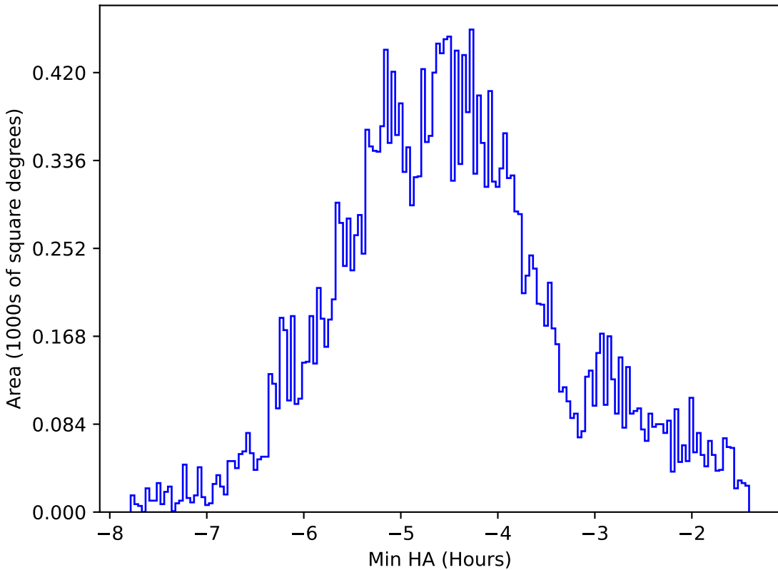
weather_cloudso2v3.4_10yrs All sky all bands: Min HA
