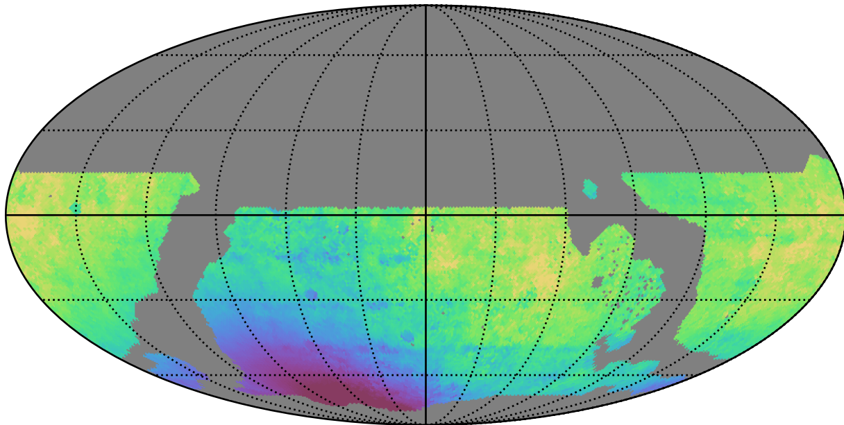
weather_cloudso2v3.4_10yrs WFD z band: Median solarElong
