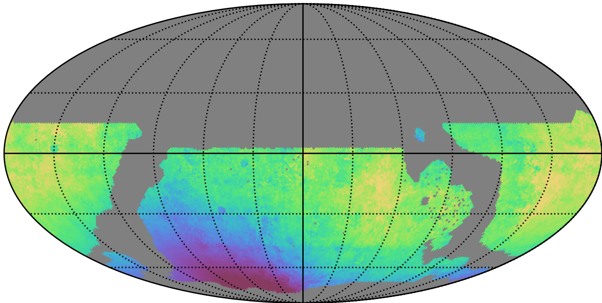
weather_cloudso2v3.4_10yrs WFD y band: Median solarElong
