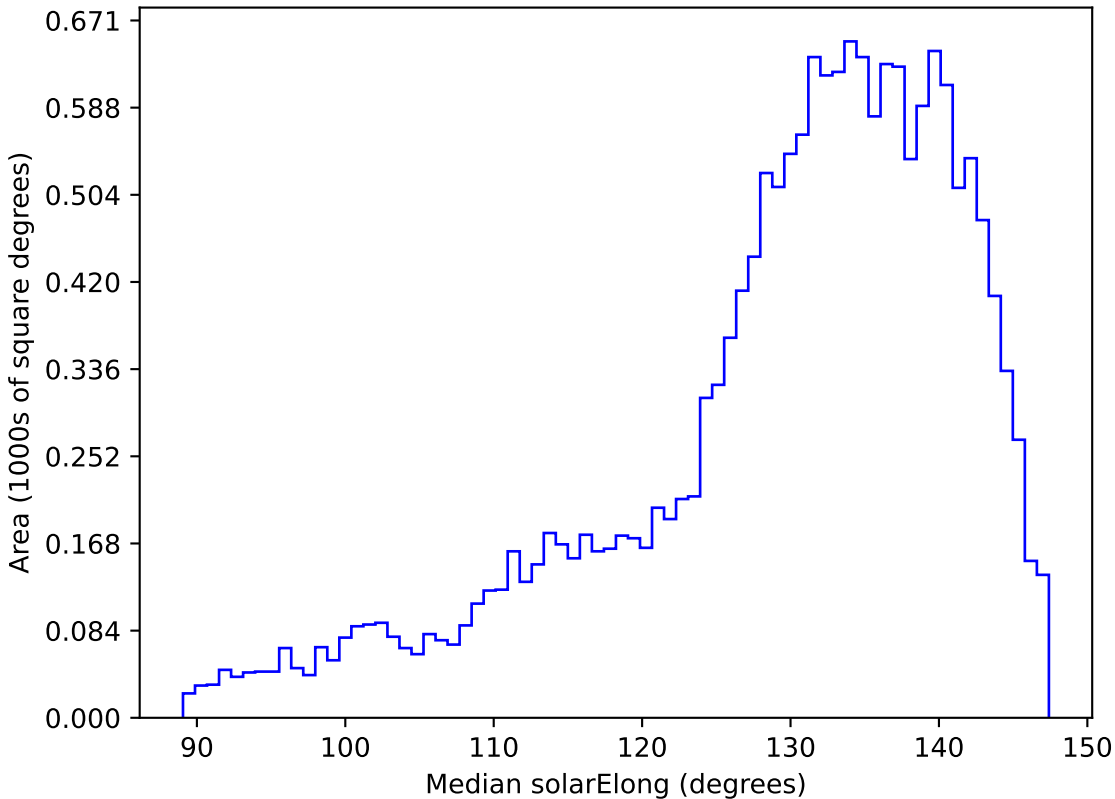
weather_cloudso2v3.4_10yrs WFD y band: Median solarElong
