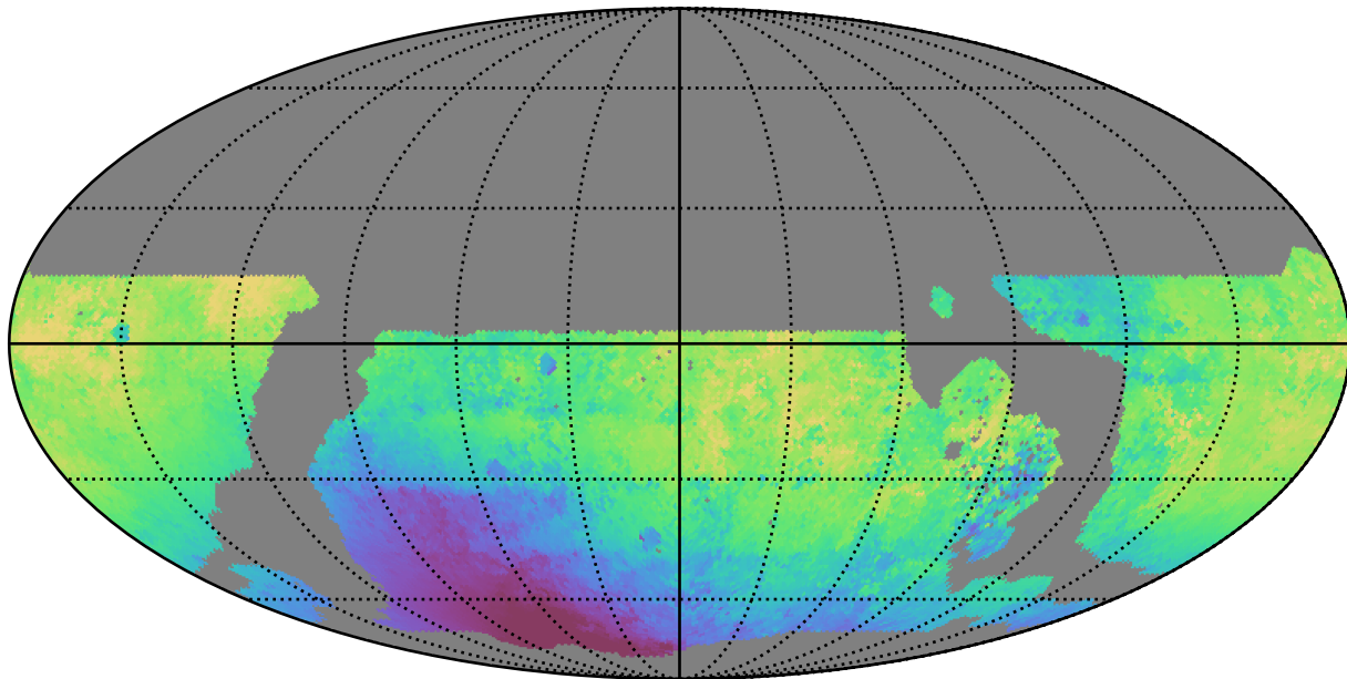
weather_cloudso2v3.4_10yrs WFD u band: Median solarElong
