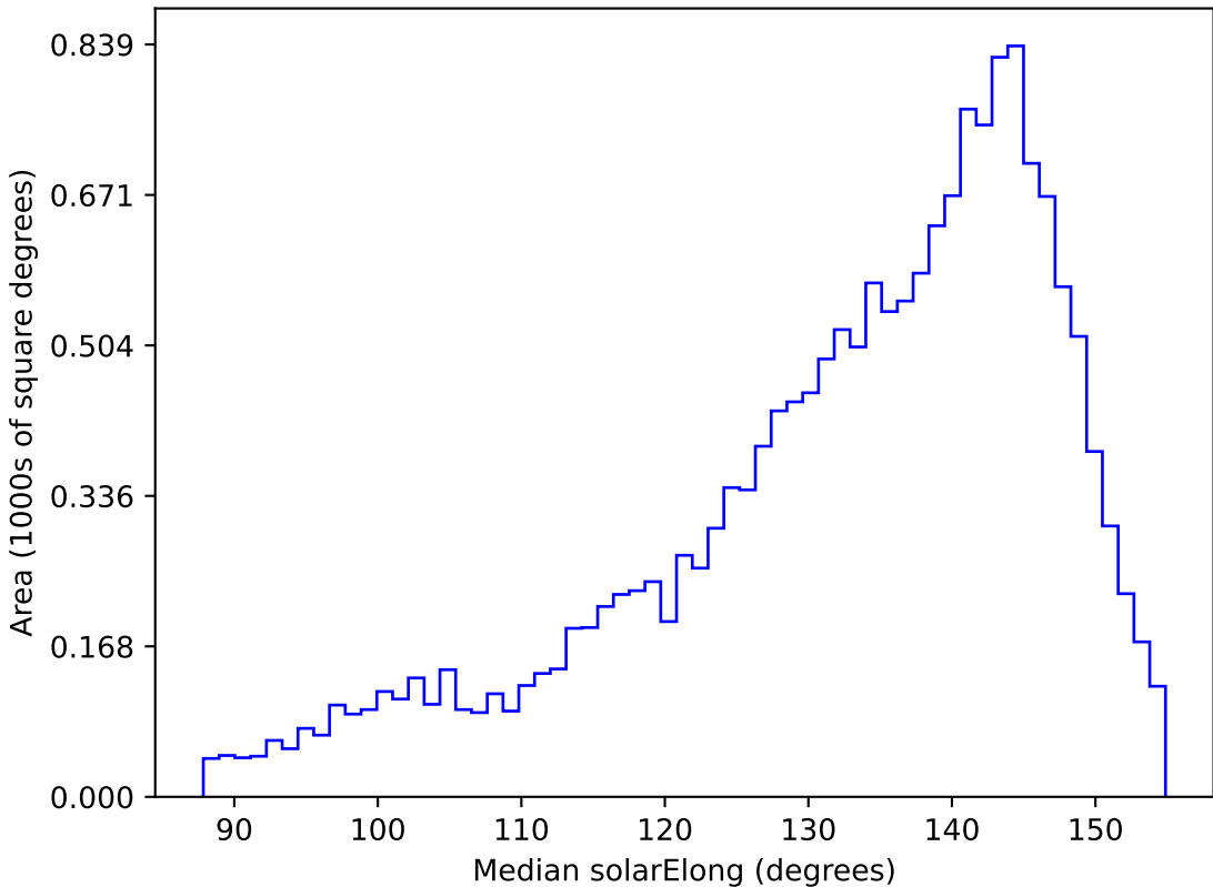
weather_cloudso2v3.4_10yrs WFD u band: Median solarElong
