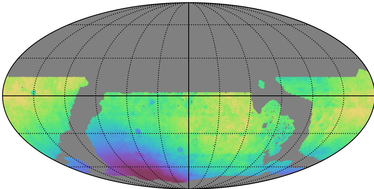
weather_cloudso2v3.4_10yrs WFD r band: Median solarElong
