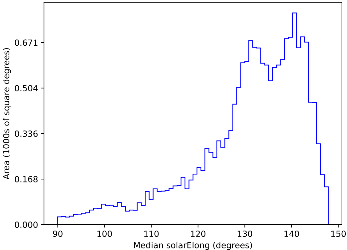
weather_cloudso2v3.4_10yrs WFD r band: Median solarElong
