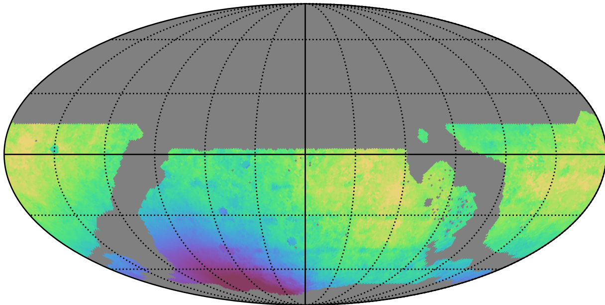
weather_cloudso2v3.4_10yrs WFD i band: Median solarElong
