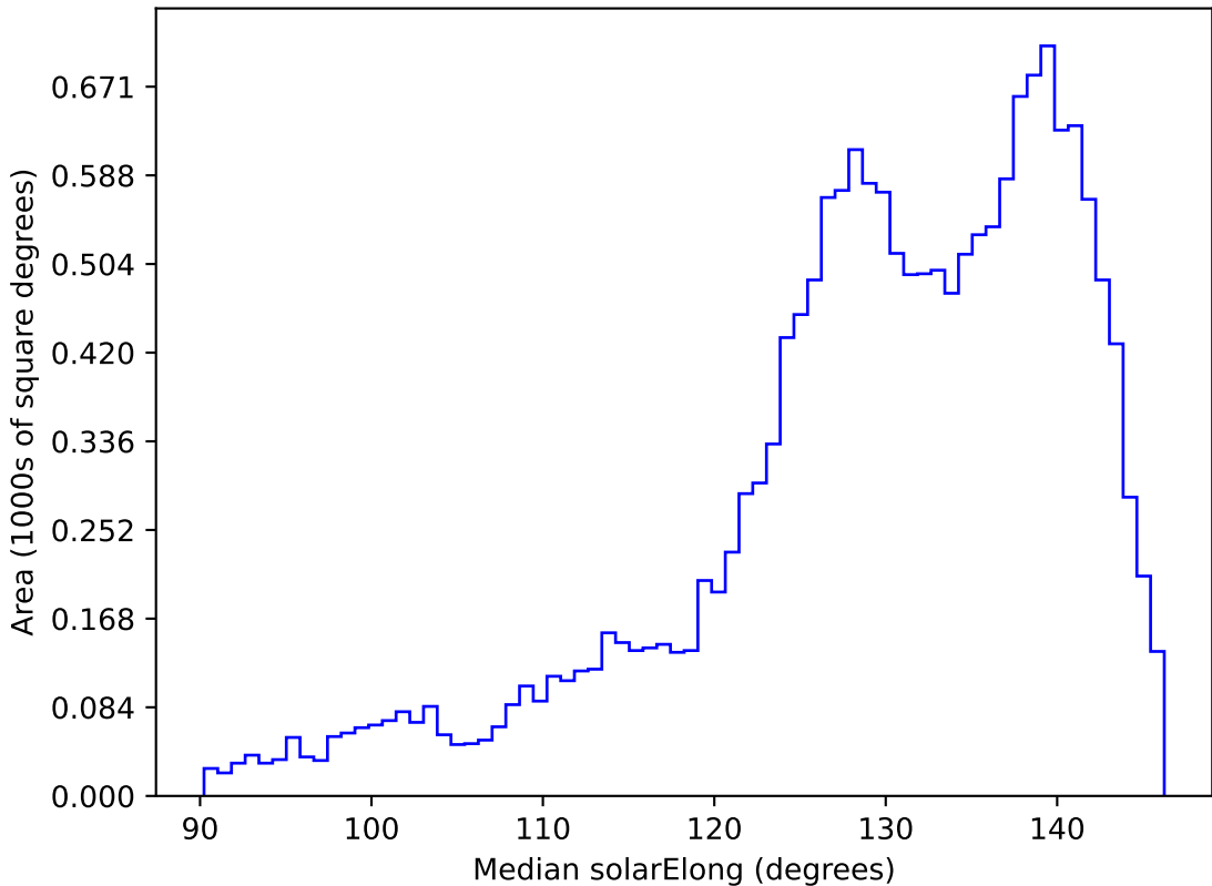
weather_cloudso2v3.4_10yrs WFD i band: Median solarElong
