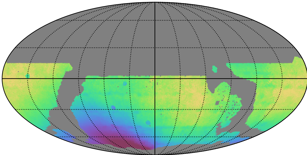
weather_cloudso2v3.4_10yrs WFD all bands: Median solarElong
