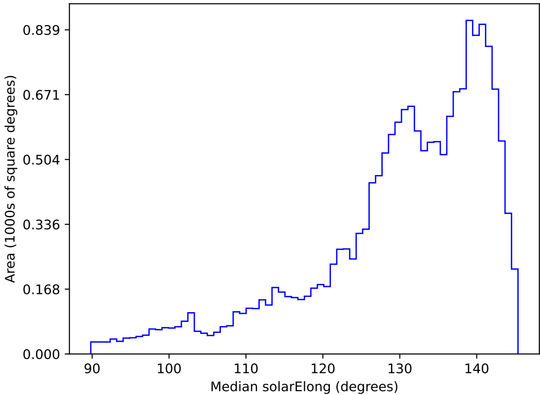
weather_cloudso2v3.4_10yrs WFD all bands: Median solarElong
