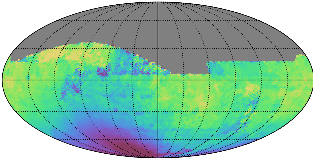
weather_cloudso2v3.4_10yrs All sky z band: Median solarElong
