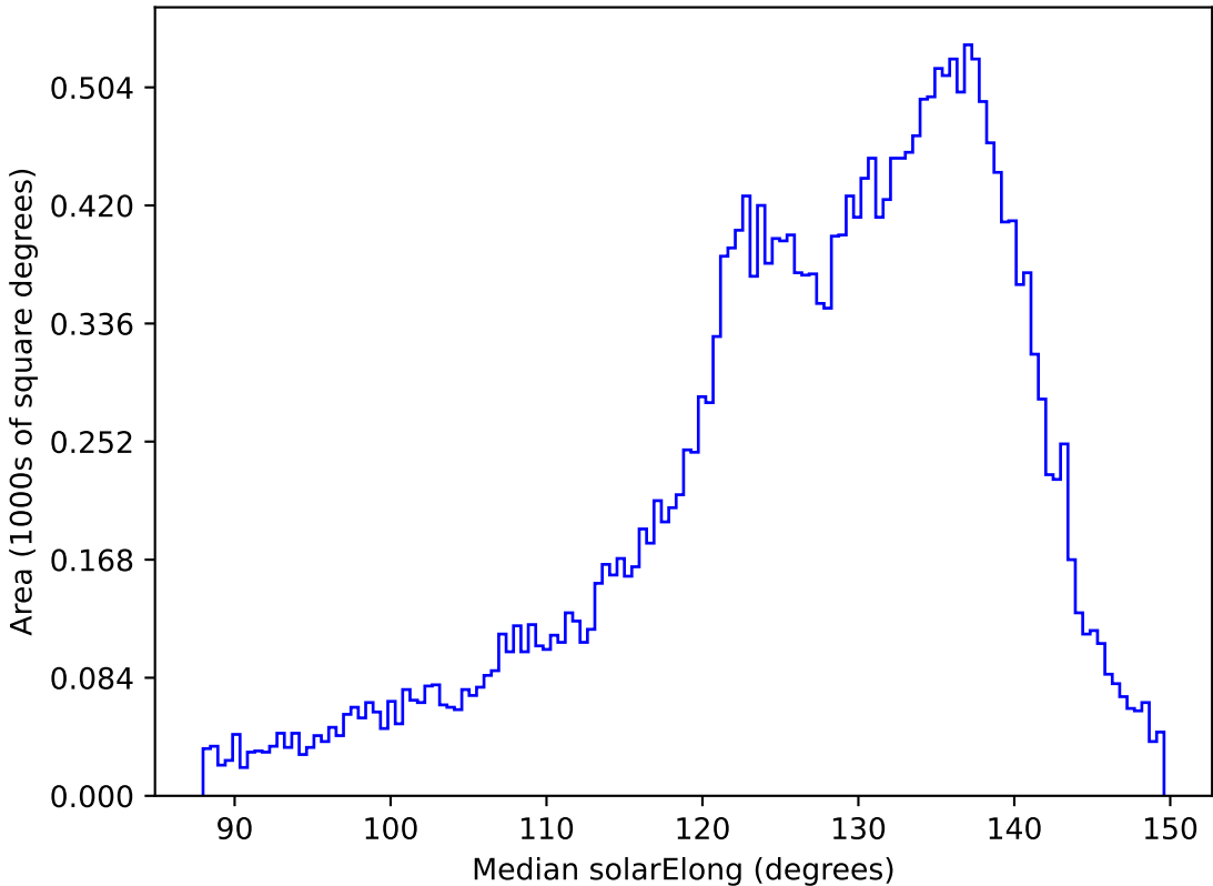
weather_cloudso2v3.4_10yrs All sky z band: Median solarElong
