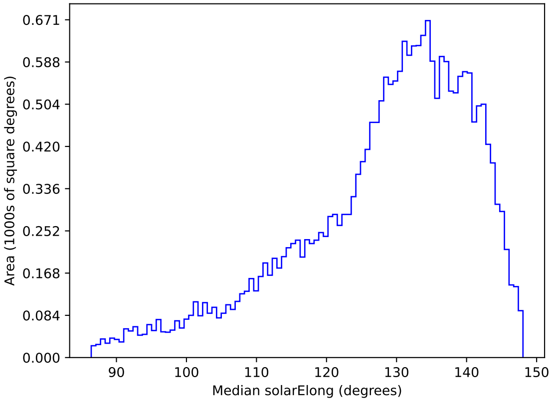
weather_cloudso2v3.4_10yrs All sky y band: Median solarElong
