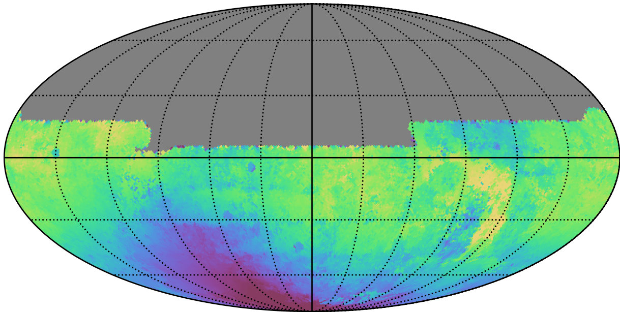
weather_cloudso2v3.4_10yrs All sky u band: Median solarElong
