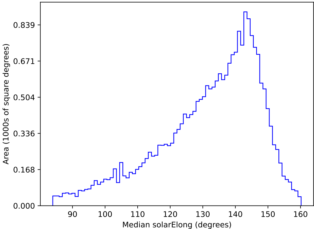
weather_cloudso2v3.4_10yrs All sky u band: Median solarElong
