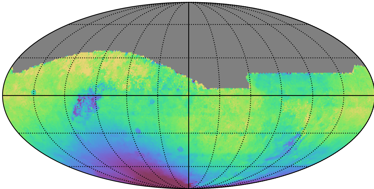
weather_cloudso2v3.4_10yrs All sky r band: Median solarElong
