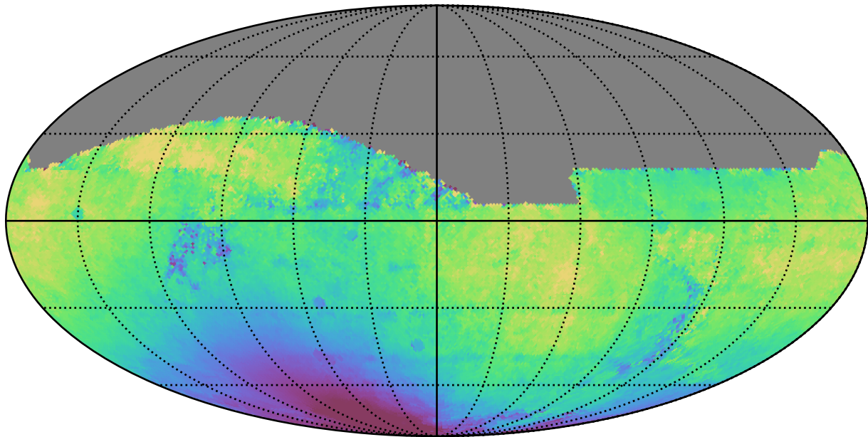
weather_cloudso2v3.4_10yrs All sky i band: Median solarElong
