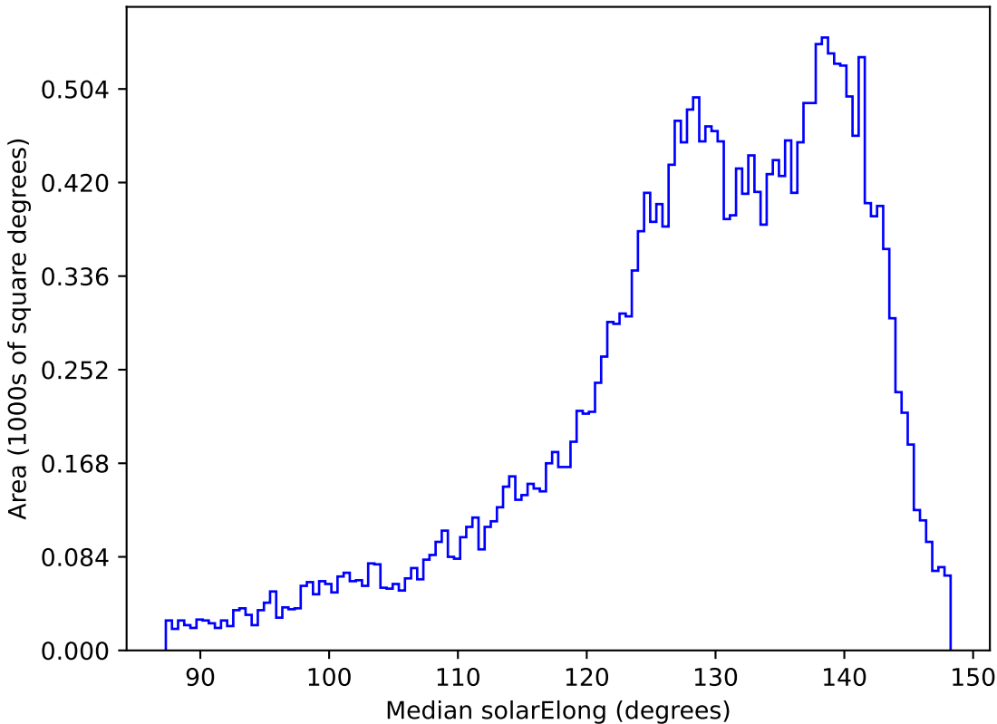
weather_cloudso2v3.4_10yrs All sky i band: Median solarElong
