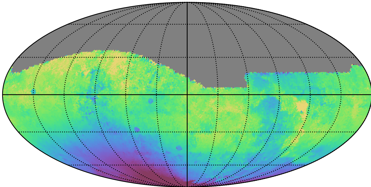
weather_cloudso2v3.4_10yrs All sky g band: Median solarElong
