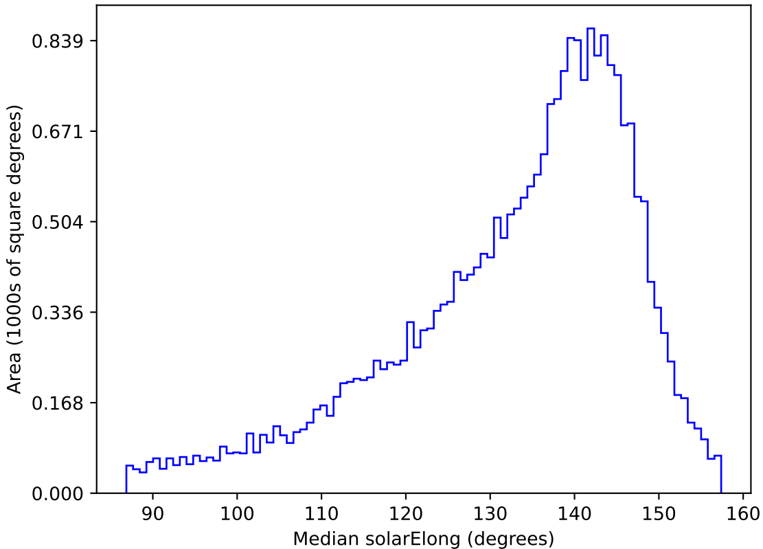
weather_cloudso2v3.4_10yrs All sky g band: Median solarElong
