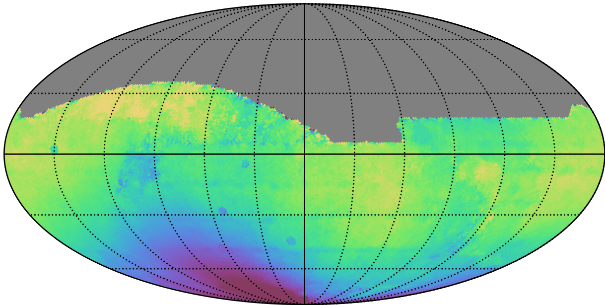
weather_cloudso2v3.4_10yrs All sky all bands: Median solarElong
