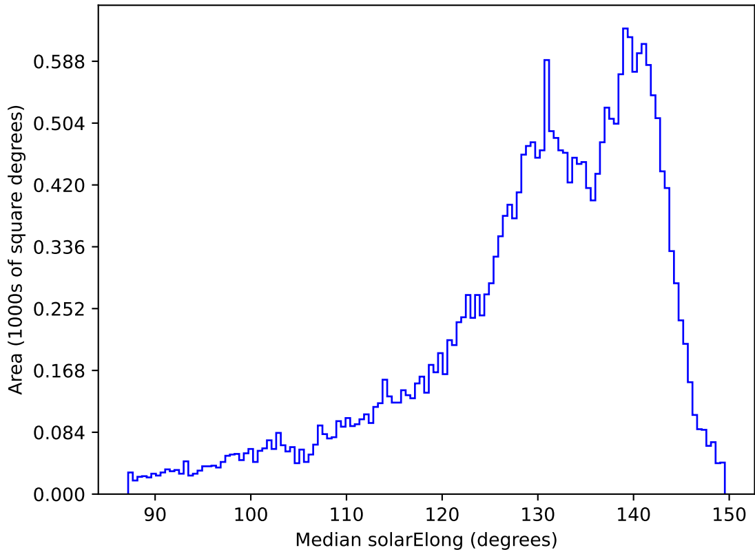
weather_cloudso2v3.4_10yrs All sky all bands: Median solarElong
