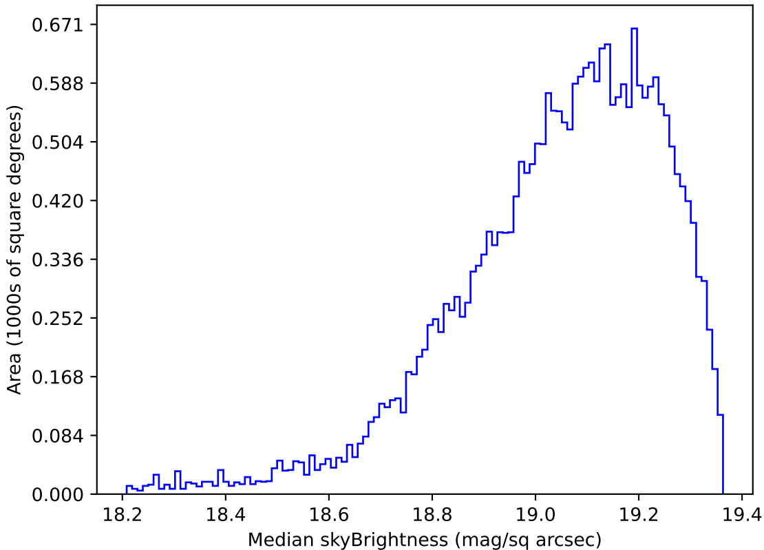
weather_cloudso2v3.4_10yrs Yr 1 z band: Median skyBrightness
