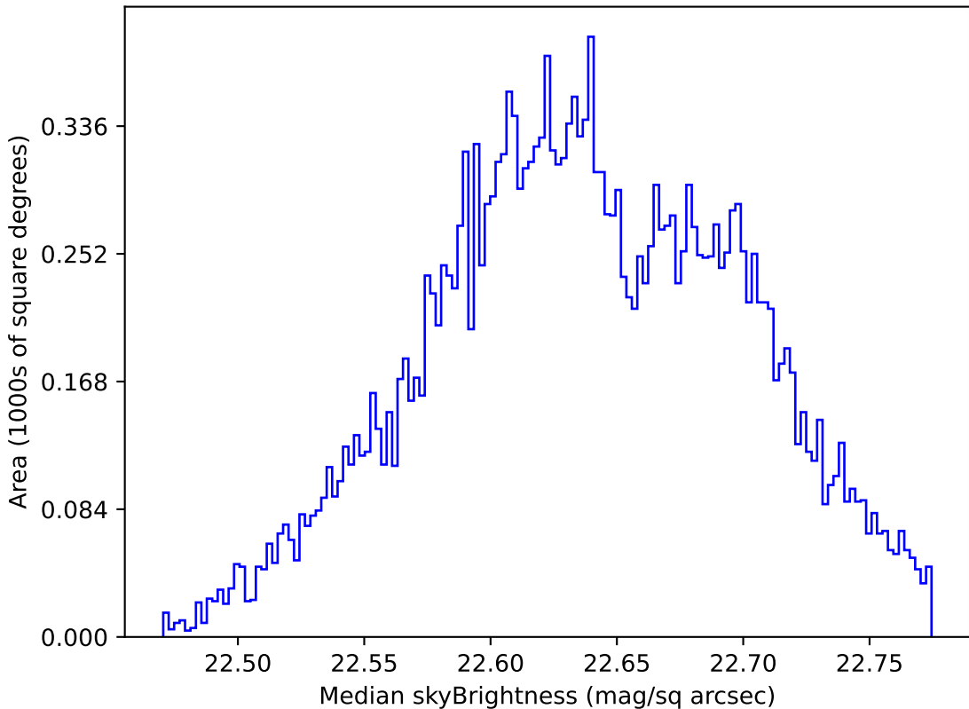
weather_cloudso2v3.4_10yrs Yr 1 u band: Median skyBrightness
