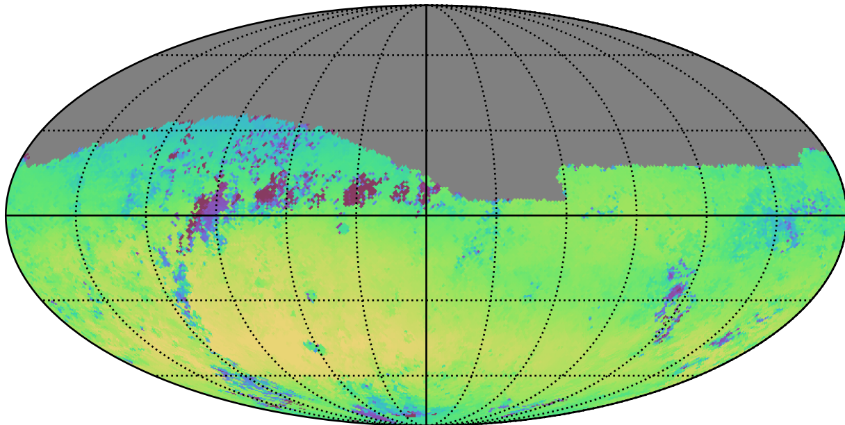
weather_cloudso2v3.4_10yrs Yr 1 r band: Median skyBrightness
