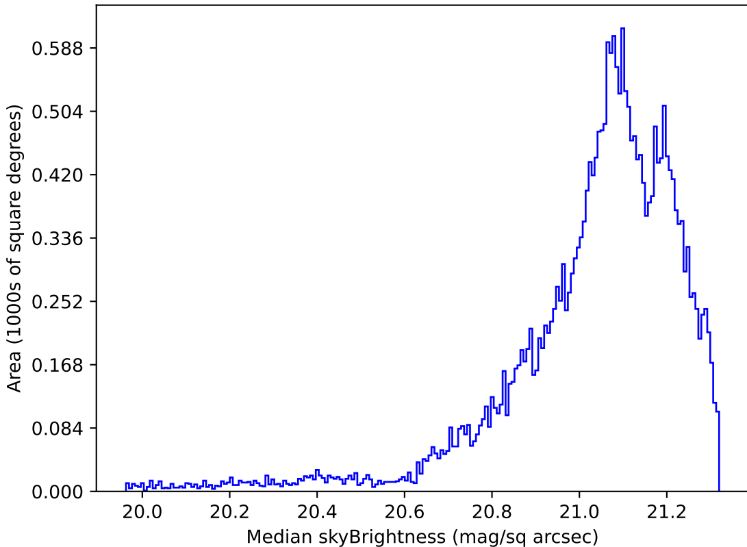
weather_cloudso2v3.4_10yrs Yr 1 r band: Median skyBrightness
