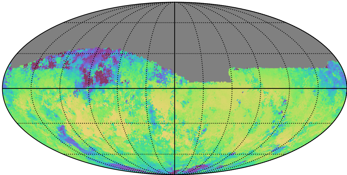
weather_cloudso2v3.4_10yrs Yr 1 i band: Median skyBrightness
