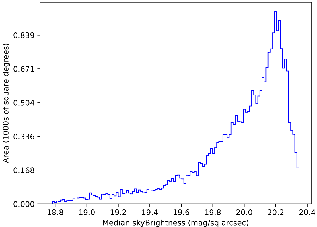
weather_cloudso2v3.4_10yrs Yr 1 i band: Median skyBrightness
