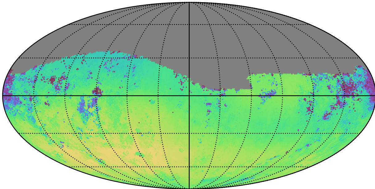
weather_cloudso2v3.4_10yrs Yr 1 g band: Median skyBrightness
