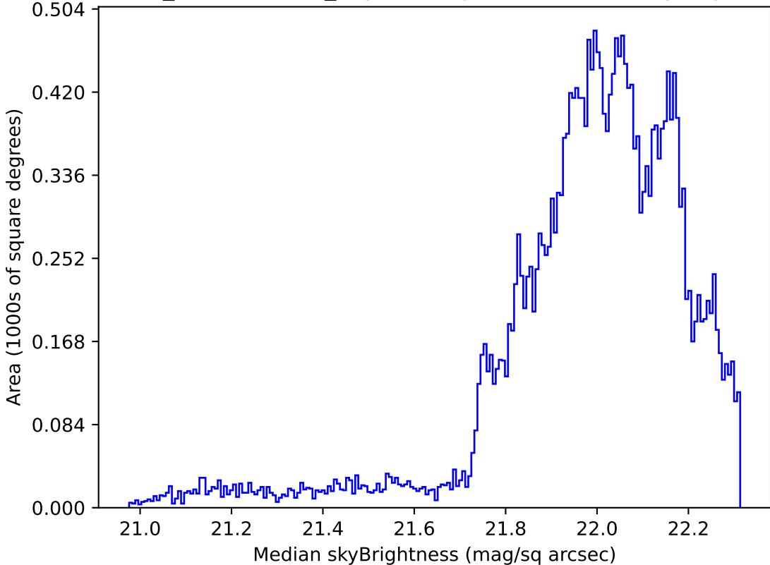
weather_cloudso2v3.4_10yrs Yr 1 g band: Median skyBrightness
