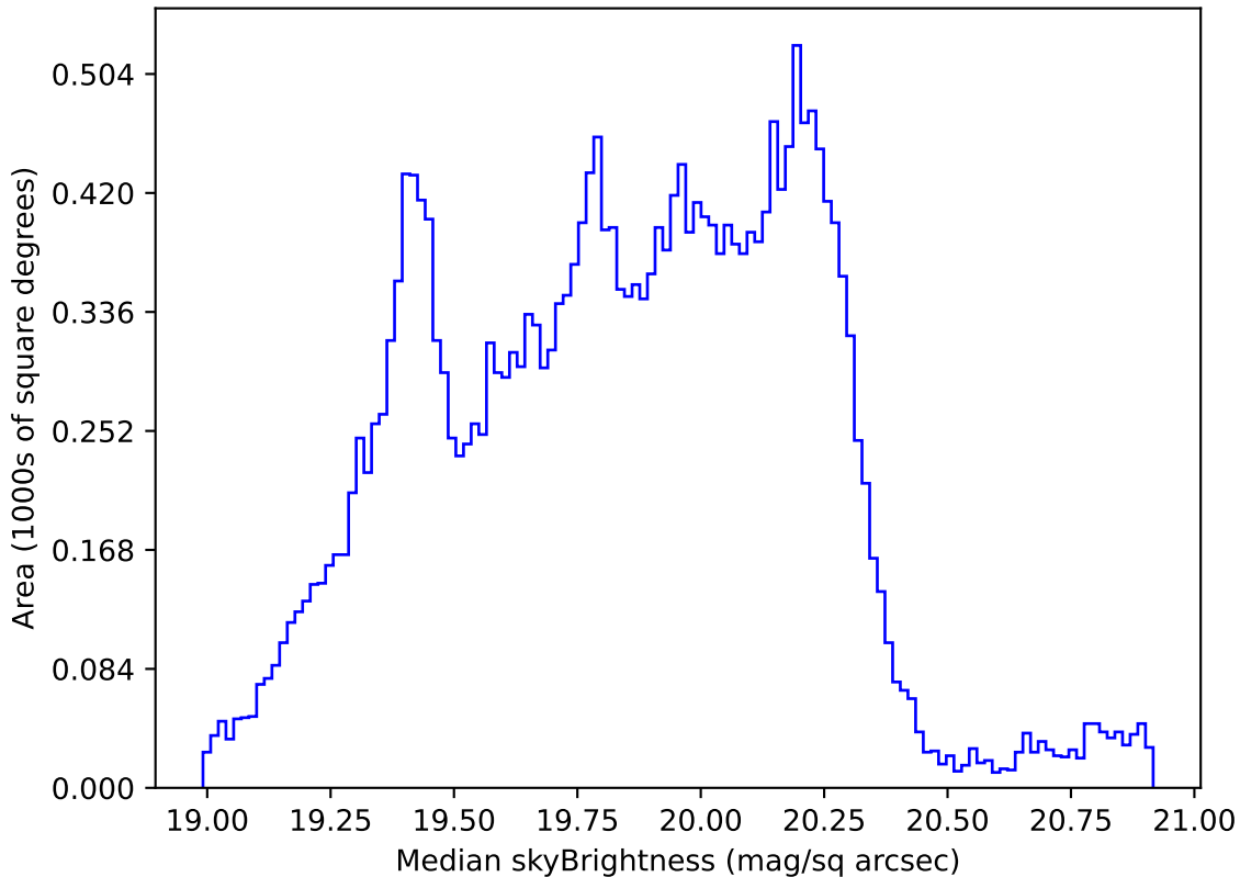
weather_cloudso2v3.4_10yrs Yr 1 all bands: Median skyBrightness
