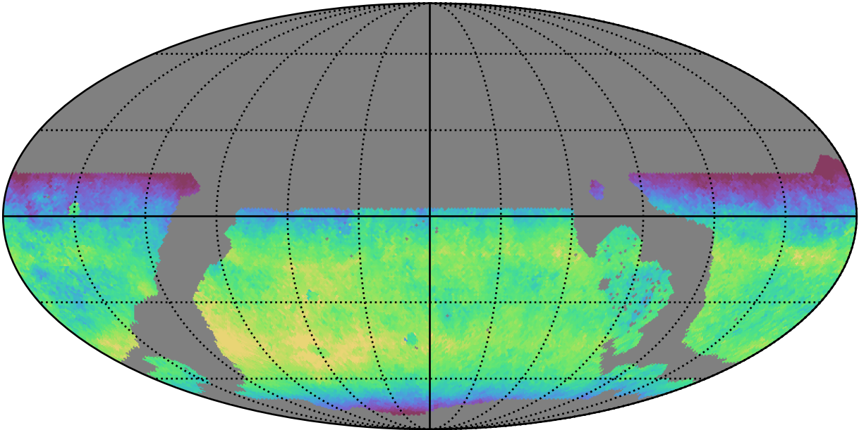
weather_cloudso2v3.4_10yrs WFD y band: Median skyBrightness
