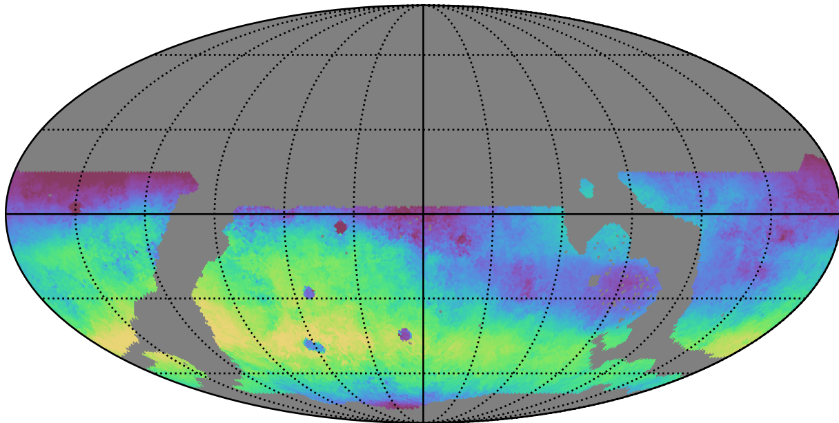
weather_cloudso2v3.4_10yrs WFD r band: Median skyBrightness
