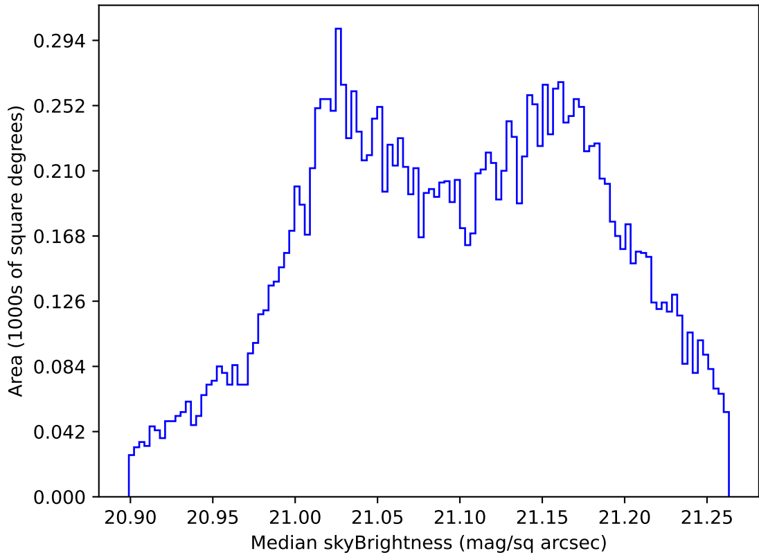
weather_cloudso2v3.4_10yrs WFD r band: Median skyBrightness
