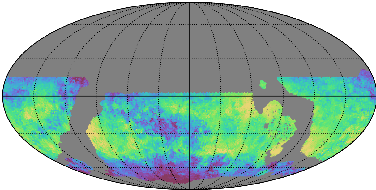
weather_cloudso2v3.4_10yrs WFD i band: Median skyBrightness
