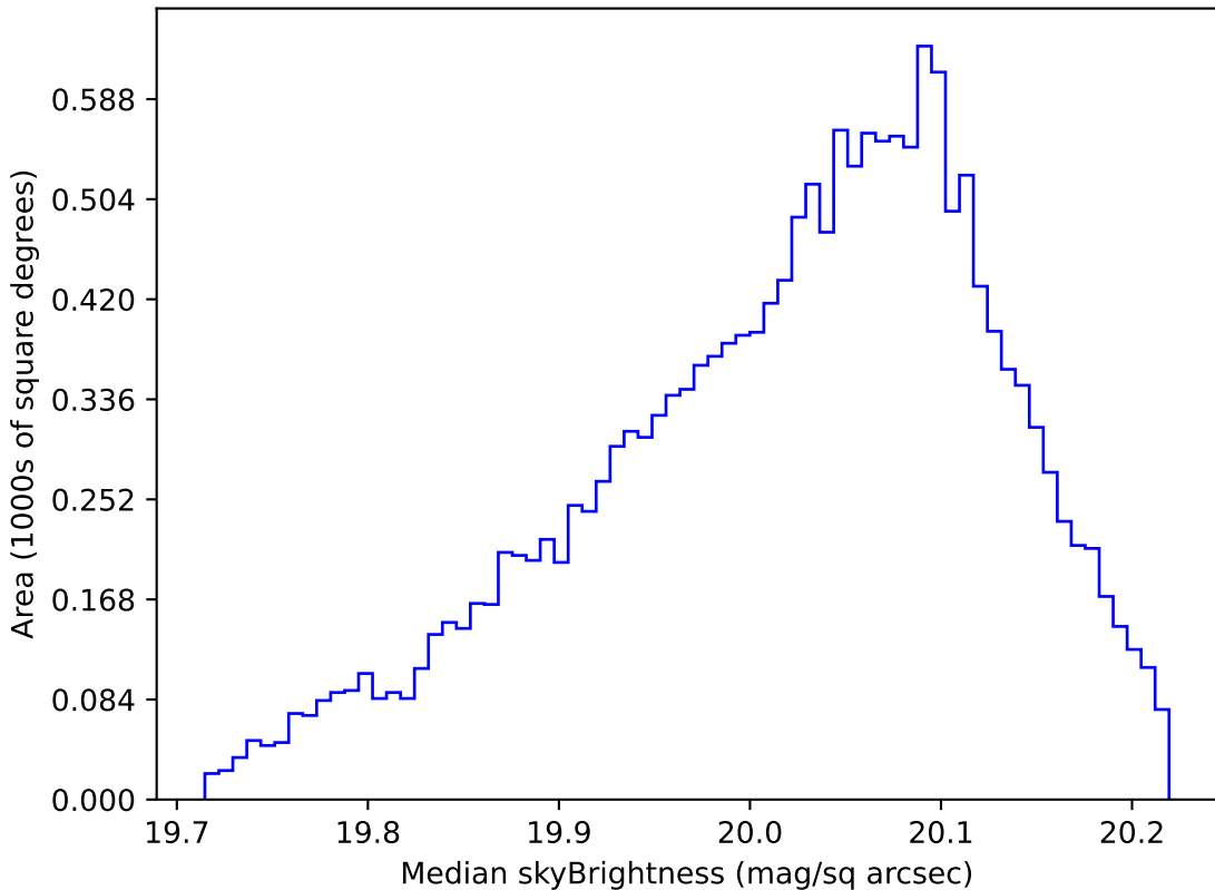
weather_cloudso2v3.4_10yrs WFD i band: Median skyBrightness
