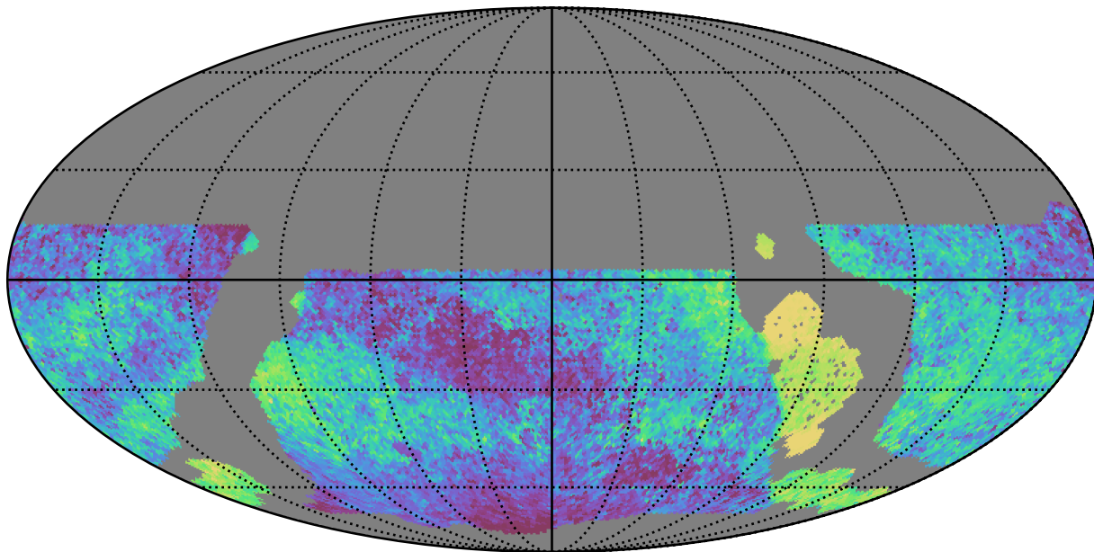
weather_cloudso2v3.4_10yrs WFD all bands: Median skyBrightness
