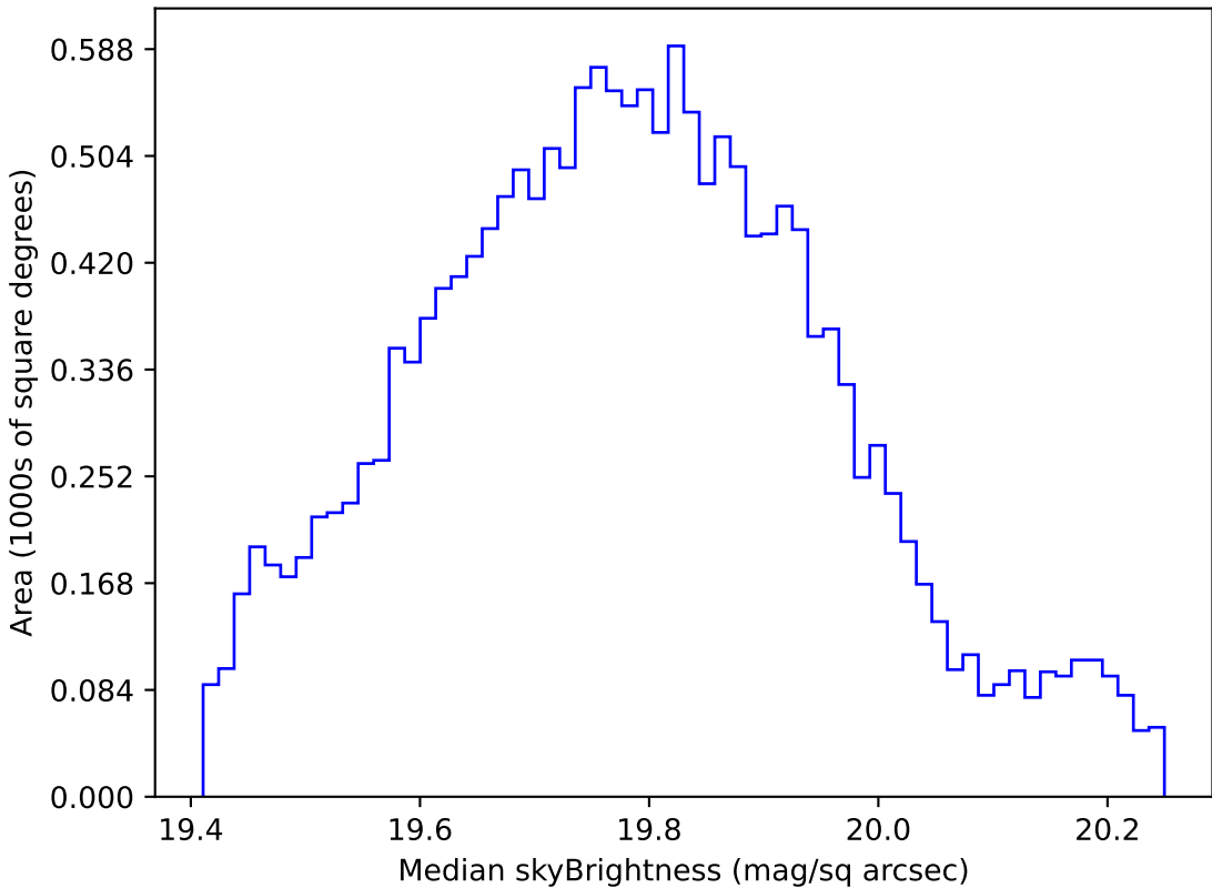
weather_cloudso2v3.4_10yrs WFD all bands: Median skyBrightness
