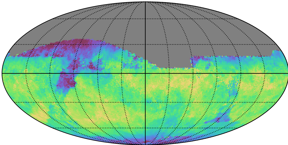
weather_cloudso2v3.4_10yrs All sky z band: Median skyBrightness
