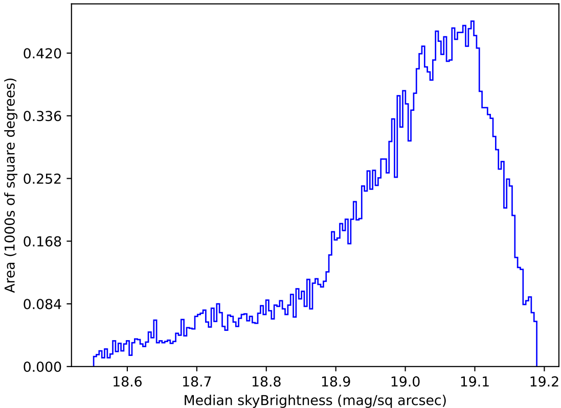
weather_cloudso2v3.4_10yrs All sky z band: Median skyBrightness
