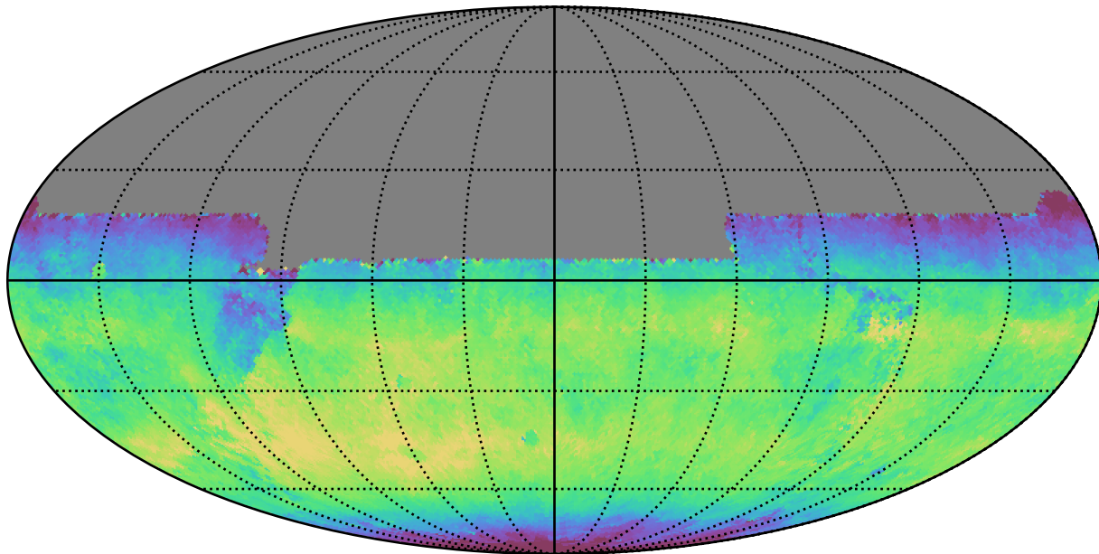
weather_cloudso2v3.4_10yrs All sky y band: Median skyBrightness
